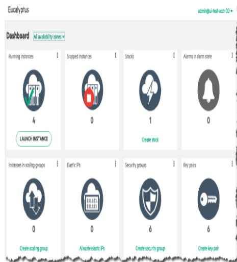
Figure 1: Eucalyptus dashboard [17].
